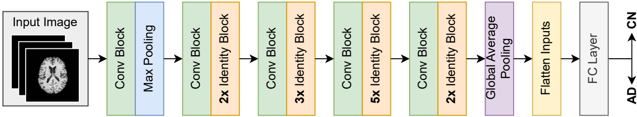
ResNet50 Model Architecture
